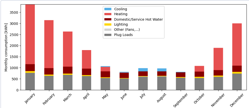
Monthly energy consumption breakdown by end use, showing the contribution of heating, cooling, lighting, domestic hot water, plug loads, and auxiliary systems throughout the year.
